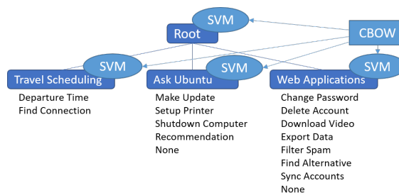
Figure 1. Hierarchy of the classes with a local hierarchical classifier per parent node.
