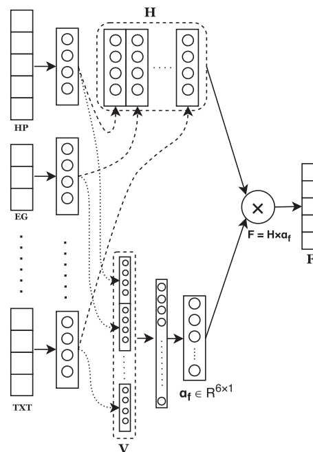
Figure 2. Attention fusion network.
