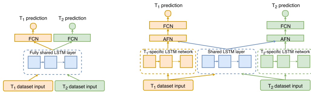
Figure 1. Fully shared (left) and shared-private (right) multitask architectures.
